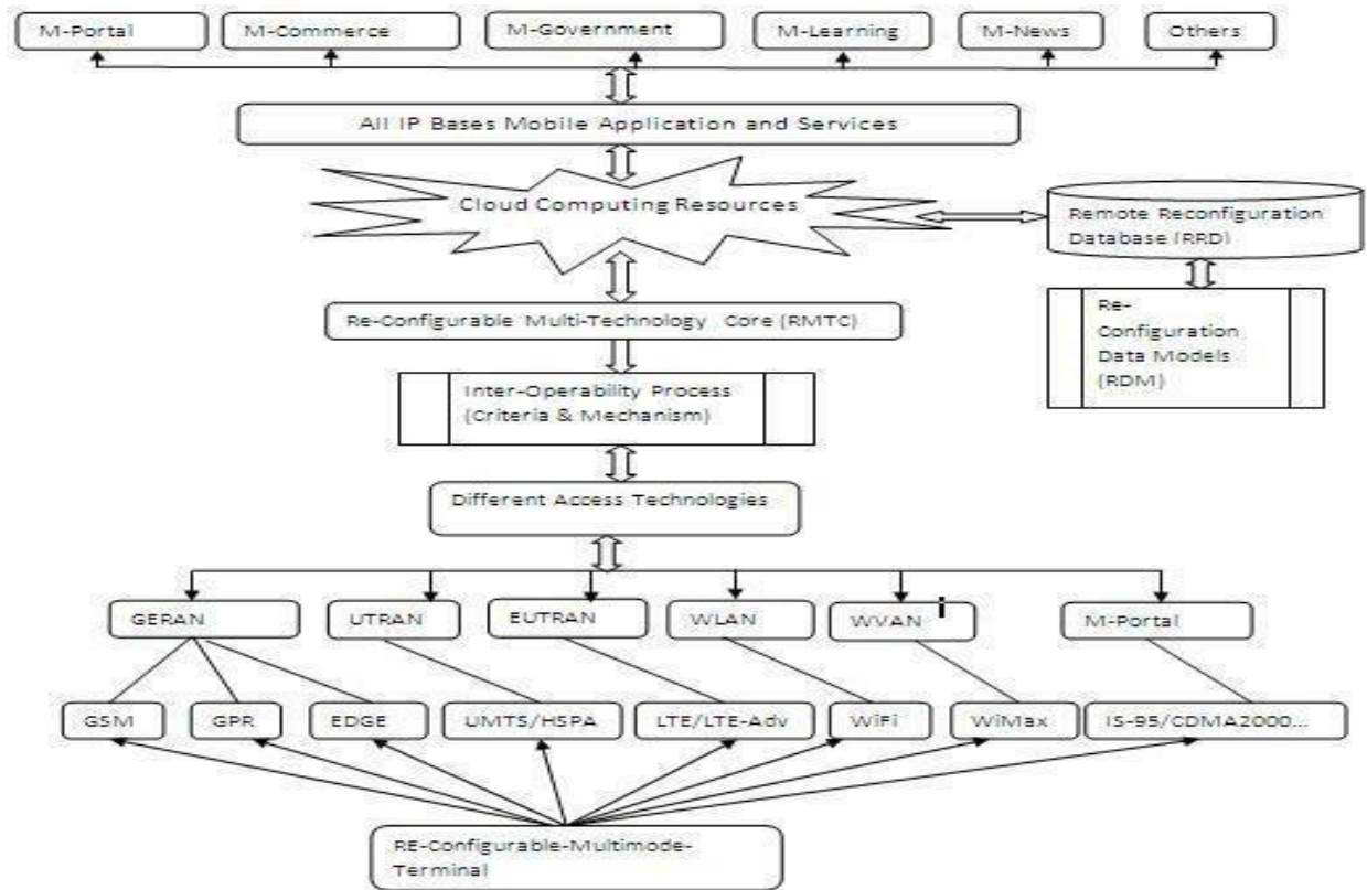
Fig. 1 5G Network Architecture[6]
