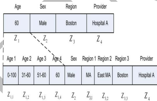
Fig.2: Index conversion- Age and region are hierarchical fields
