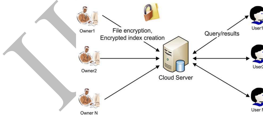
Fig. 1: Architecture of proposed work
